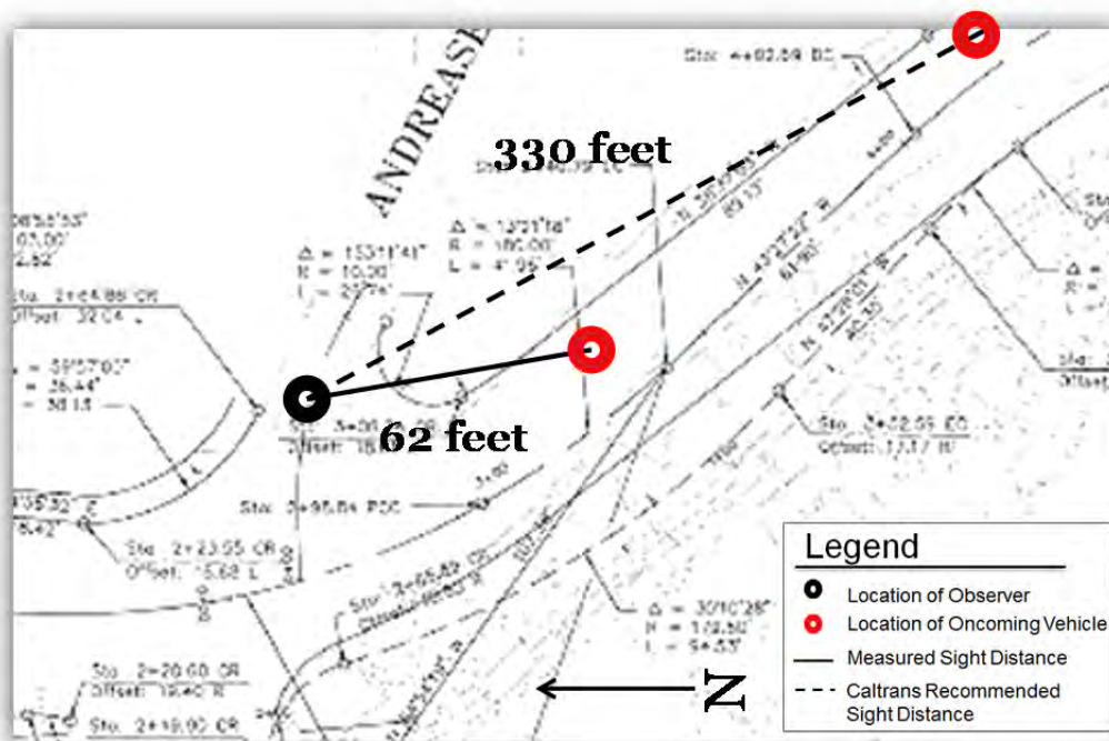
Figure 19: Andreason Drive Sight Distance
