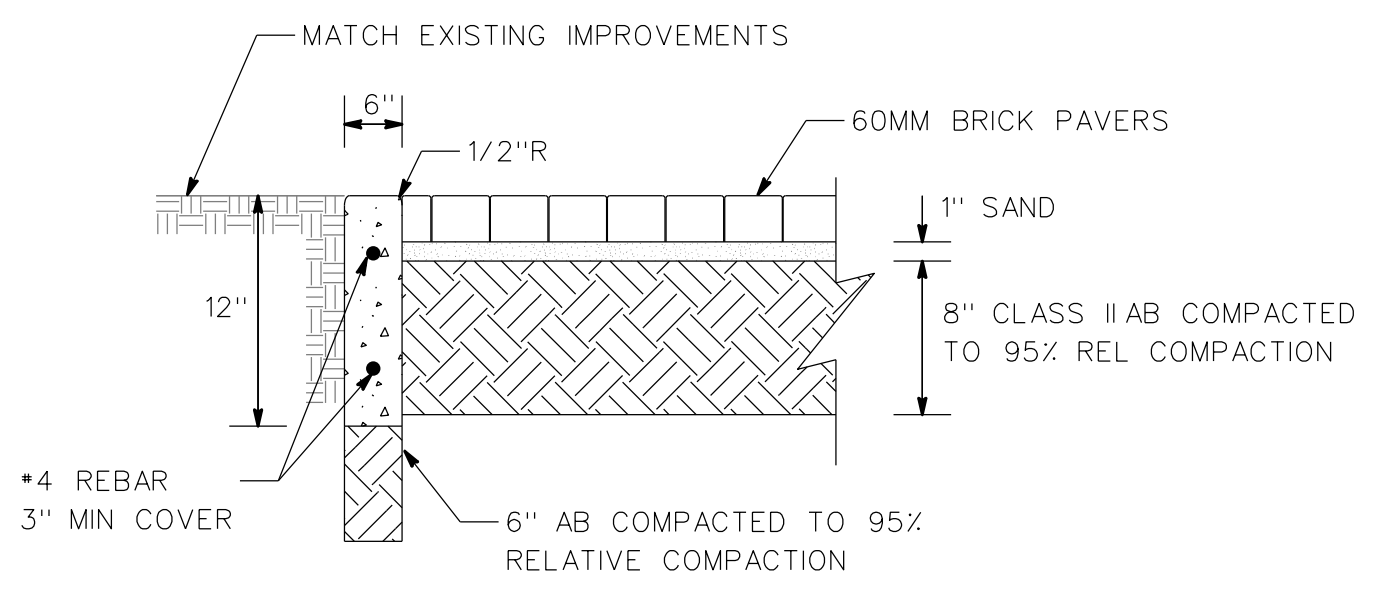
5 2 FLUSH CURB AND TYPICAL PAVER DETAIL NTS
