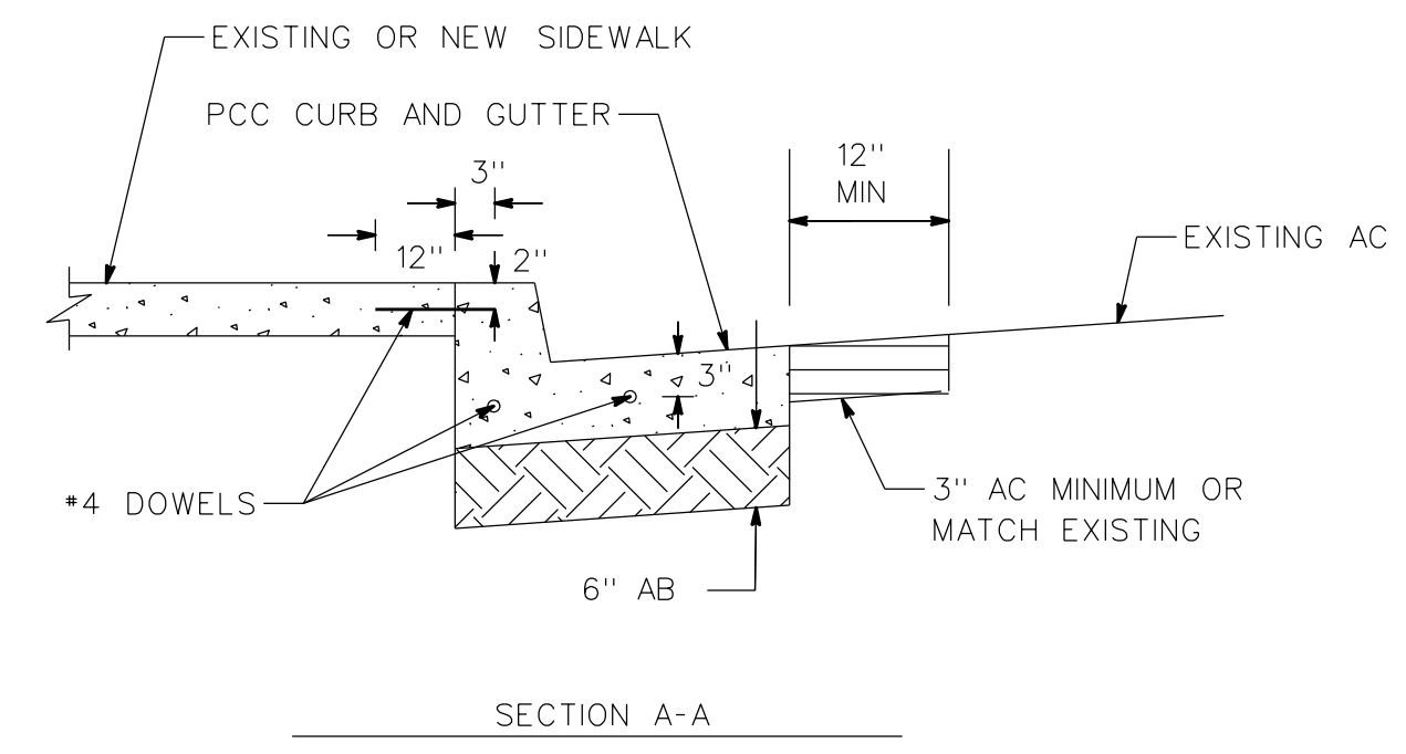
1 2 REPLACEMENT CURB AND GUTTER DETAIL NTS
