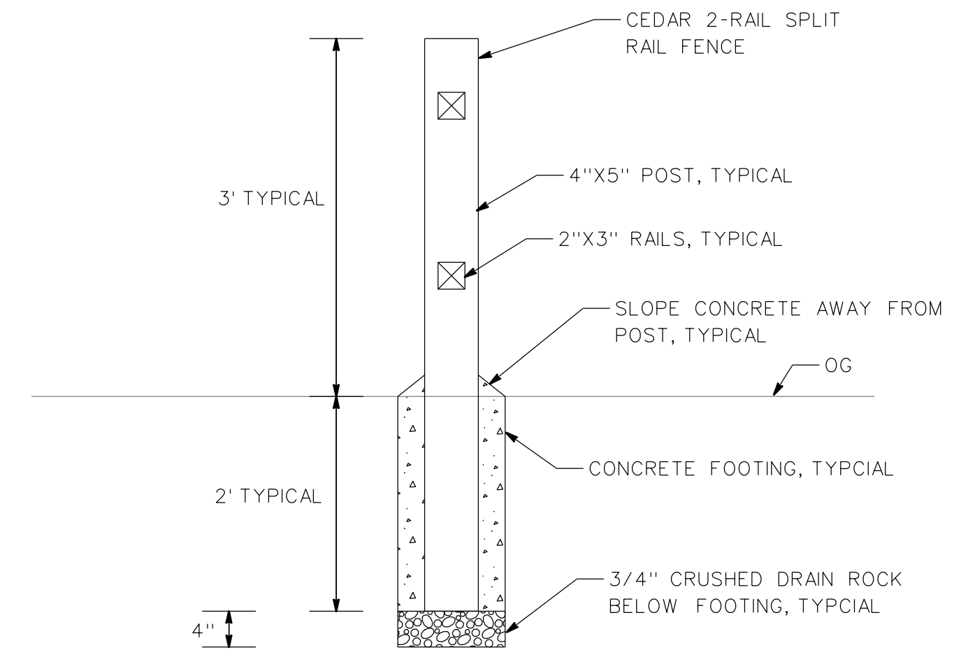
7 2 CEDAR SPLIT RAIL FENCE DETAIL NTS
