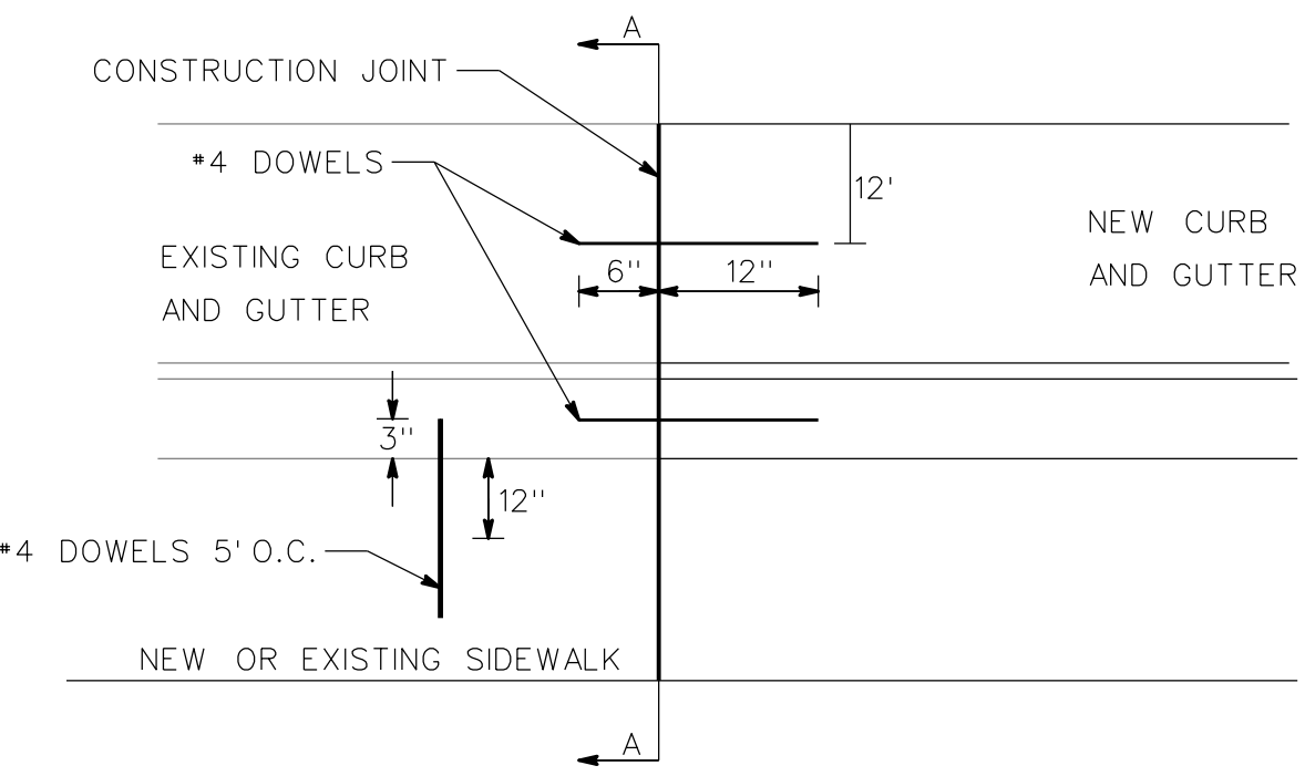
1 2 REPLACEMENT CURB AND GUTTER DETAIL NTS
