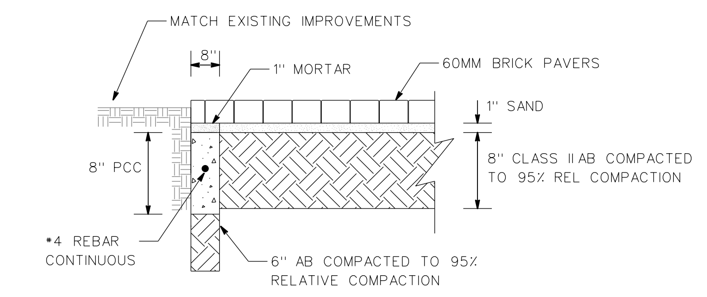
6 2 PAVER SUPPORT CURB AND TYPICAL PAVER DETAIL NTS
