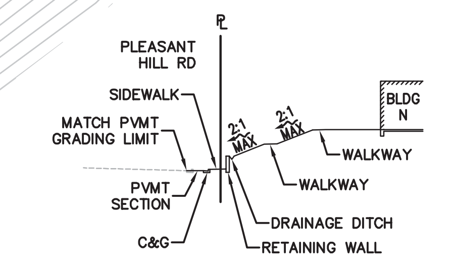
A SECTION NTS
