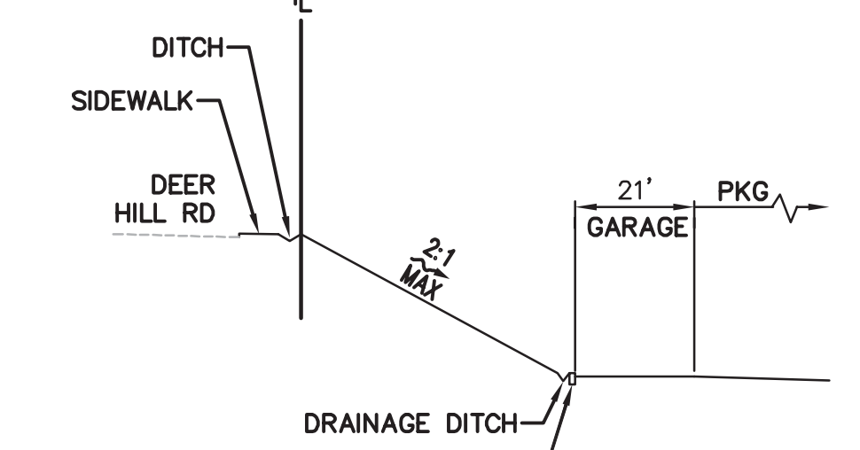
F SECTION NTS
