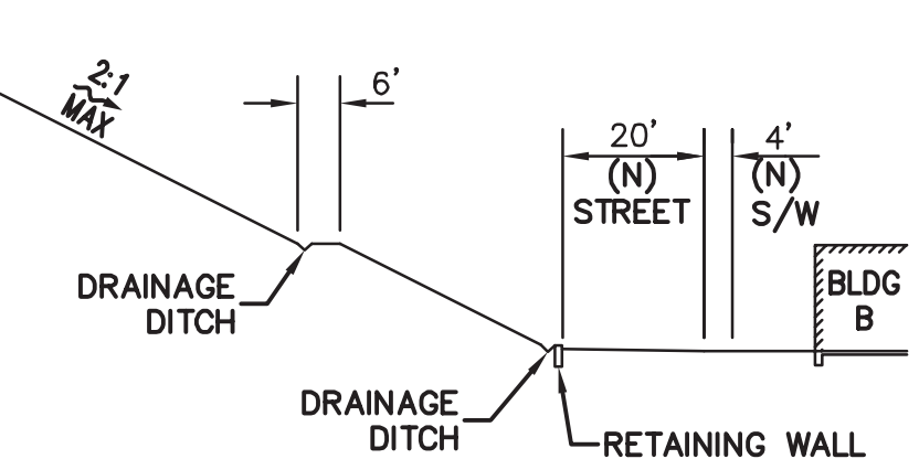
D SECTION NTS
