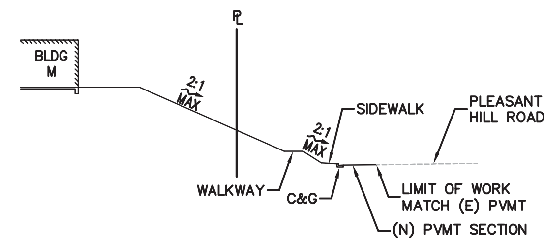
C SECTION NTS
