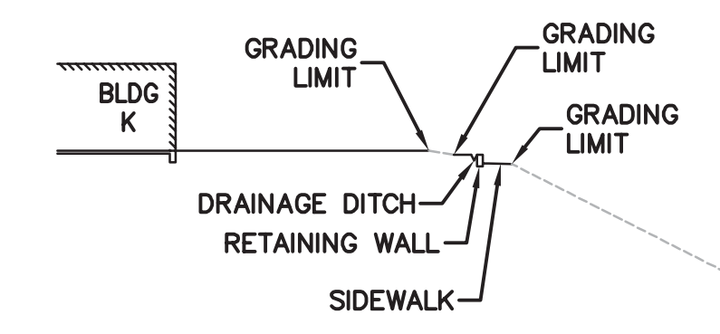
E SECTION NTS
