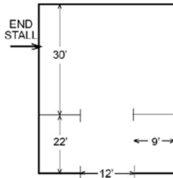
PARALLEL (0°) PARKING
