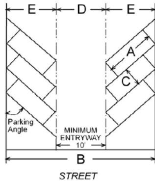
30° - 45° - 60° PARKING
