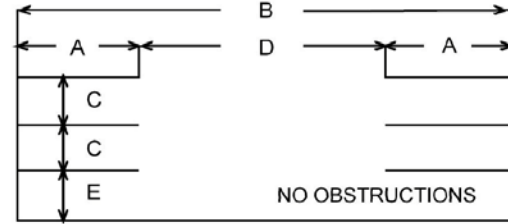
90° PARKING
