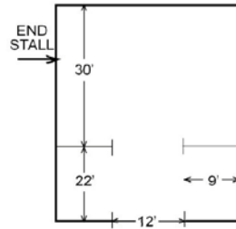
PARALLEL (0°) PARKING
